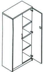
RE-908 Wardrobe L800 x W400 x H1730
