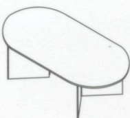
NY-CF 2400 Conference Table L2400 x W1200 x H750 mm
